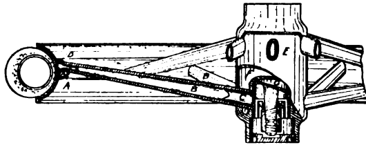
FIG. 66.—Part Sectional View of a Tubular Steel Wheel, used on many automobiles of all powers. Although, to the date of the present writing, the principal issue among authorities is upon the respective merits of wood and wire wheels, this type of wheel is steadily growing in favor. Among the advantages claimed are: superior strength to either wire or wood; true, balanced running, as a pulley on a shaft; practical immunity to rust, on account of the inner and outer brass coating on hubs and spokes and the brazing at all joints; ability to stand the twist and tension of severe strains in the transmission of power; rims formed from a continuous tube; spokes made from high carbon cycle tubing, oval in shape and reinforced at both hub and rim; perfect alignment secured by assembling all parts in jigs. As shown in the cut, the parts are: A, tubular steel rim; B, tubular steel spokes; C, tubular steel reinforcement at hub; D, tubular steel reinforcement at rim; E, outer tubular steel hub shell; F, middle tubular steel hub shell; G, inner hub shell over axle spindle. The method of securing the hub to the axle is also shown. Although, as must be fairly obvious, such a construction admits of very little sidewise spring action under stress of travel or collision, which is a particularly desirable feature in wooden wheels, especially with steel tires, the slant of the spokes effectually prevents such extreme deformation as would tend to disable a wood or wire wheel. The oval shape of the spoke tubes, and their arrangement as regards both hub and rim, enable the carrying of greater loads, in proportion to weight, than are possible with other varieties of wheel. It is also possible to keep such wheels perfectly clean, without risk of injury by rust, as must result from attempts to wash wire wheels, as already stated. Furthermore, tubular steel wheels do not shrink when dry, as do wooden wheels, and, consequently, require no process of soaking to restore them to normal condition.
